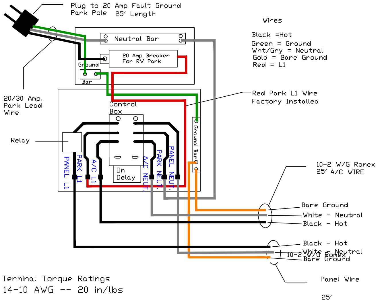
JTB POWER SOLUTION WIRING DIAGRAM
